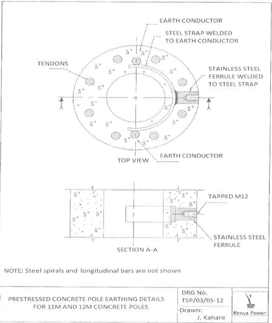
Fig. 2 – Concrete pole earthing details
